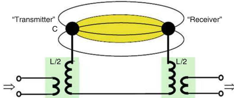
Fig. 6.14 Interpretation as an open resonant circuit
